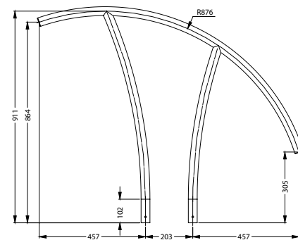
Artisan Series Hand Rail (ART-1001-MG Standard/ART-1001S-MGF Flanged)
