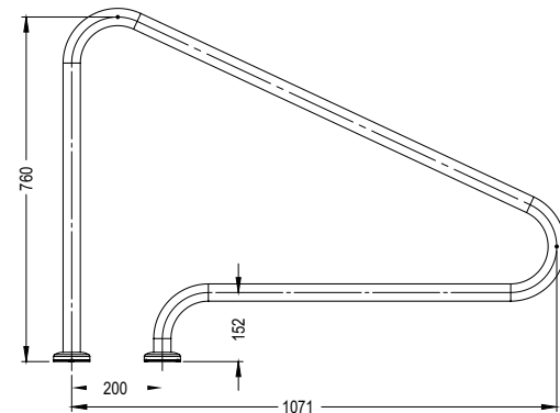
Deck Mounted Stair Rail (SR-DS Standard/SR-DF Flanged)
