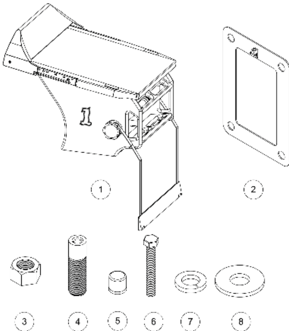
Figure 2 | Velocity Advantage Parts
