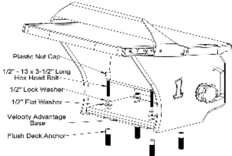
Figure 6 | Mounting Hardware
